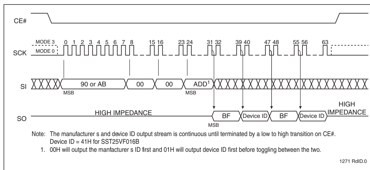
Figure 21: Read-ID Sequence
